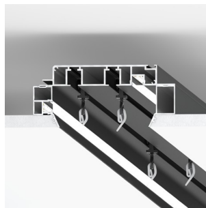
UMBRA Curtain track of 115 mm width
