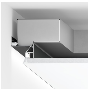
UMBRA Floating ceiling with a ventilation perforation hole
