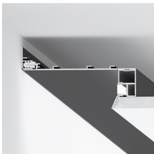
UMBRA Floating ceiling with an adjustable gap
