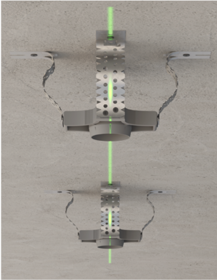
The versatility of the solution allows you to install a frameless light in both PVC and fabric ceilings. The embedded structure is grey, located 10 mm above the canvas and is not translucent.
