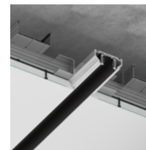
Installation in one layer of drywall
