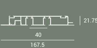
CURTAIN TRACK PROFILE 140 MM
